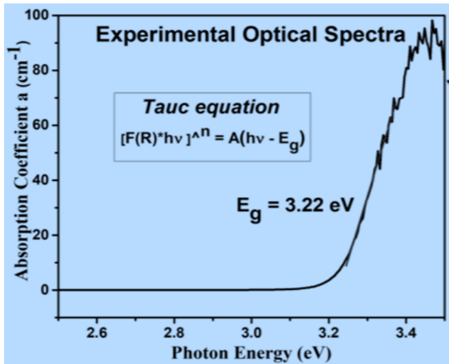
Absorption spectra of BaTiO 3 using DRS
