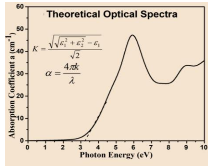
Absorption spectra of BaTiO 3 using density functional theory(DFT)
