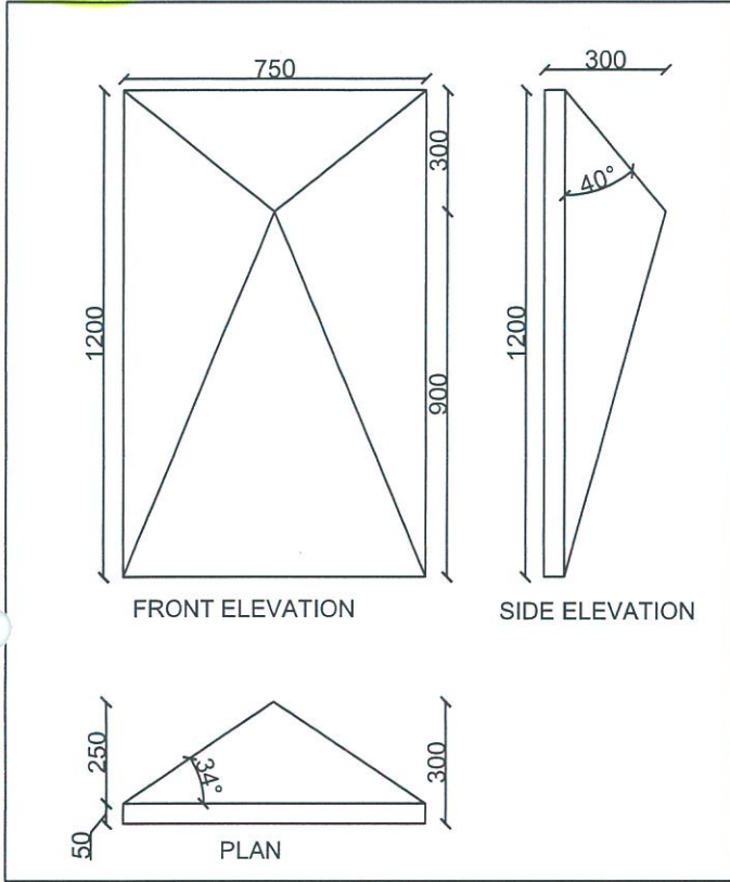
TYPE A - 750 WIDTH - 750mm X 1200mm X 300mm
