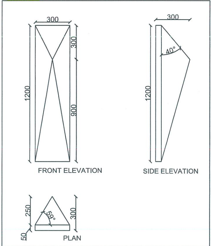
TYPE D - 300 WIDTH - 300mm X 1200mm X 300mm
