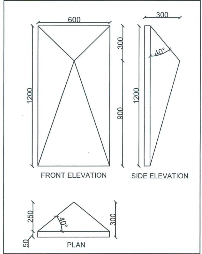
TYPE B - 600 WIDTH - 600mm X 1200mm X 300mm
