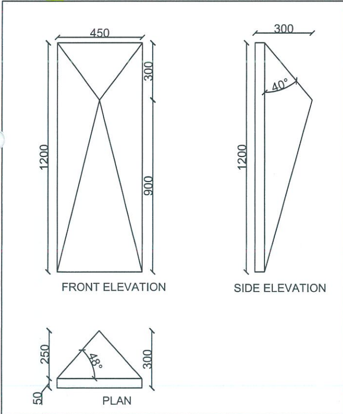
TYPE C - 450 WIDTH - 450mm X 1200mm X 300mm
